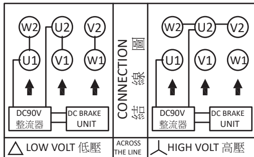
6 條結線附煞車整流器 6 Lead With Rectifier
