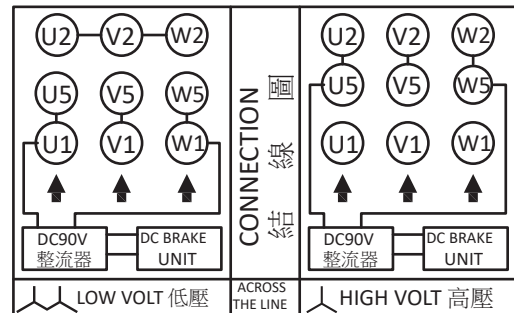
9 條結線附煞車整流器 9 Lead With Rectifier
