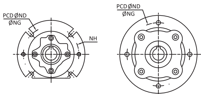
IEC-B14
